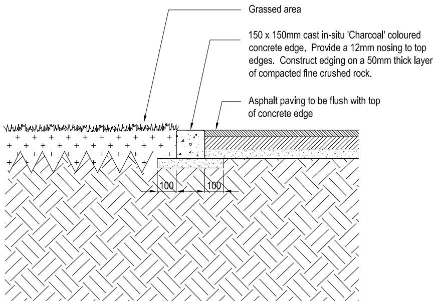
Section: Edge of grassed area and asphalt paving
