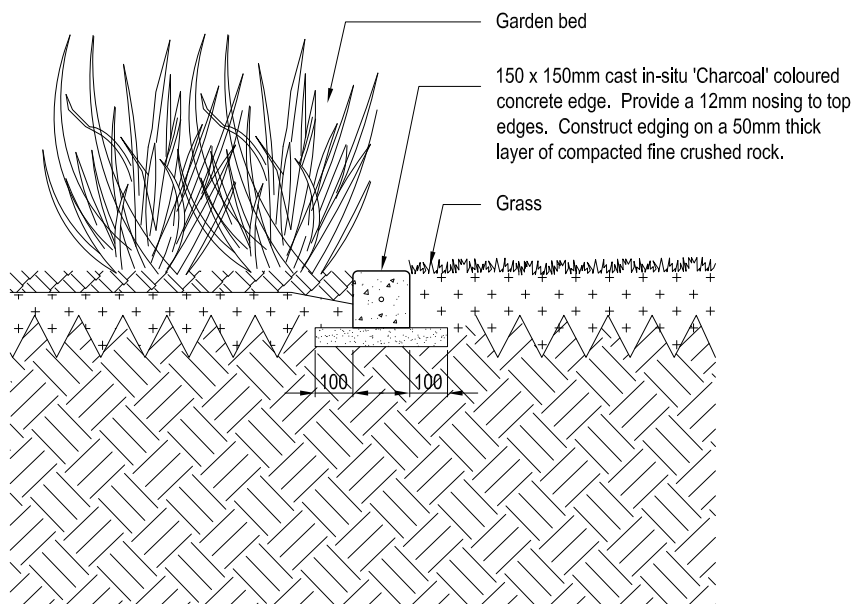
Section: Edge of garden bed and grass
