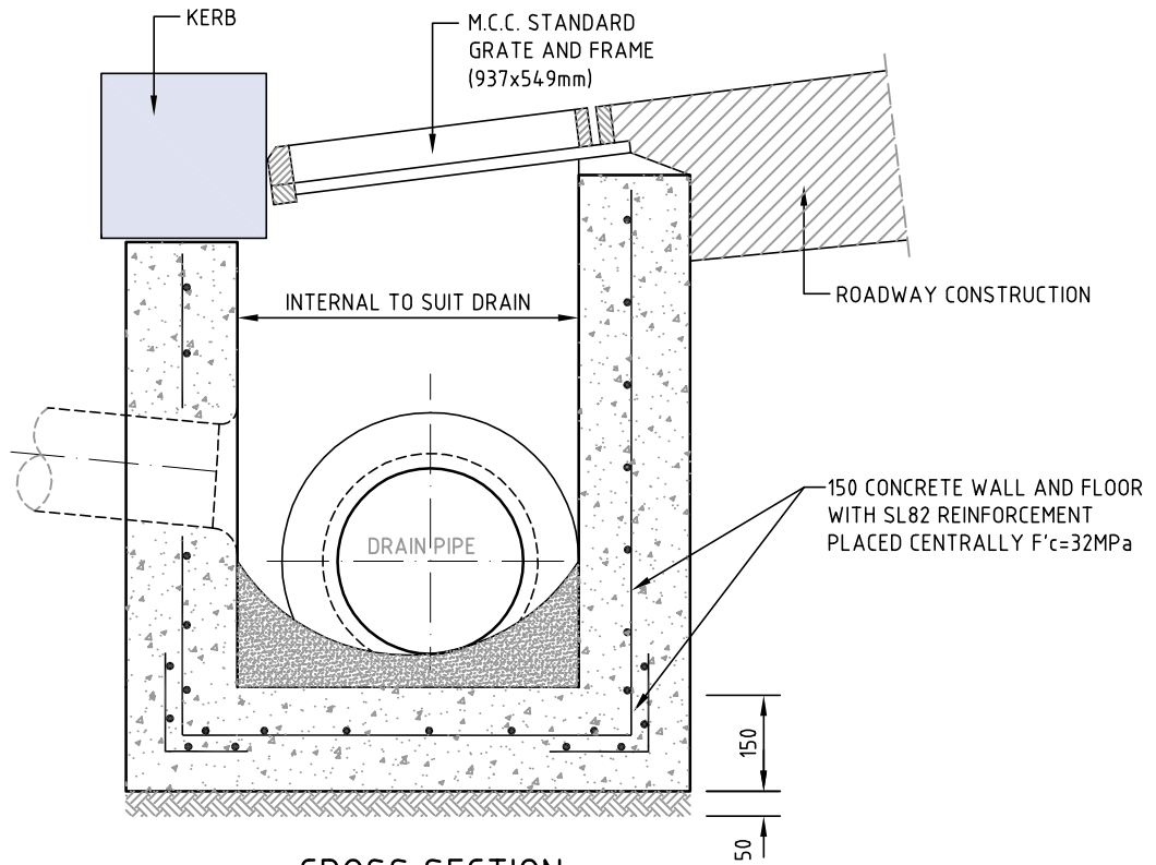
CROSS SECTION
