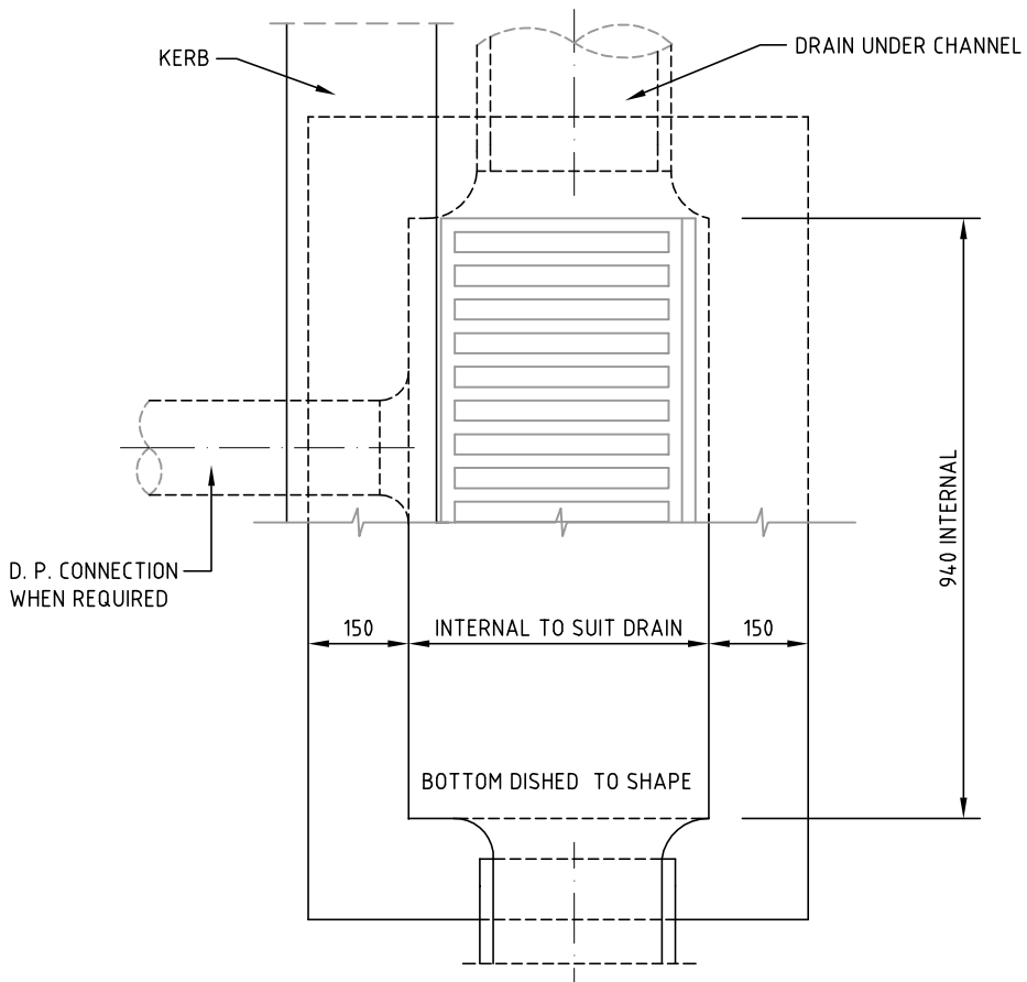
PLAN AND SECTION
