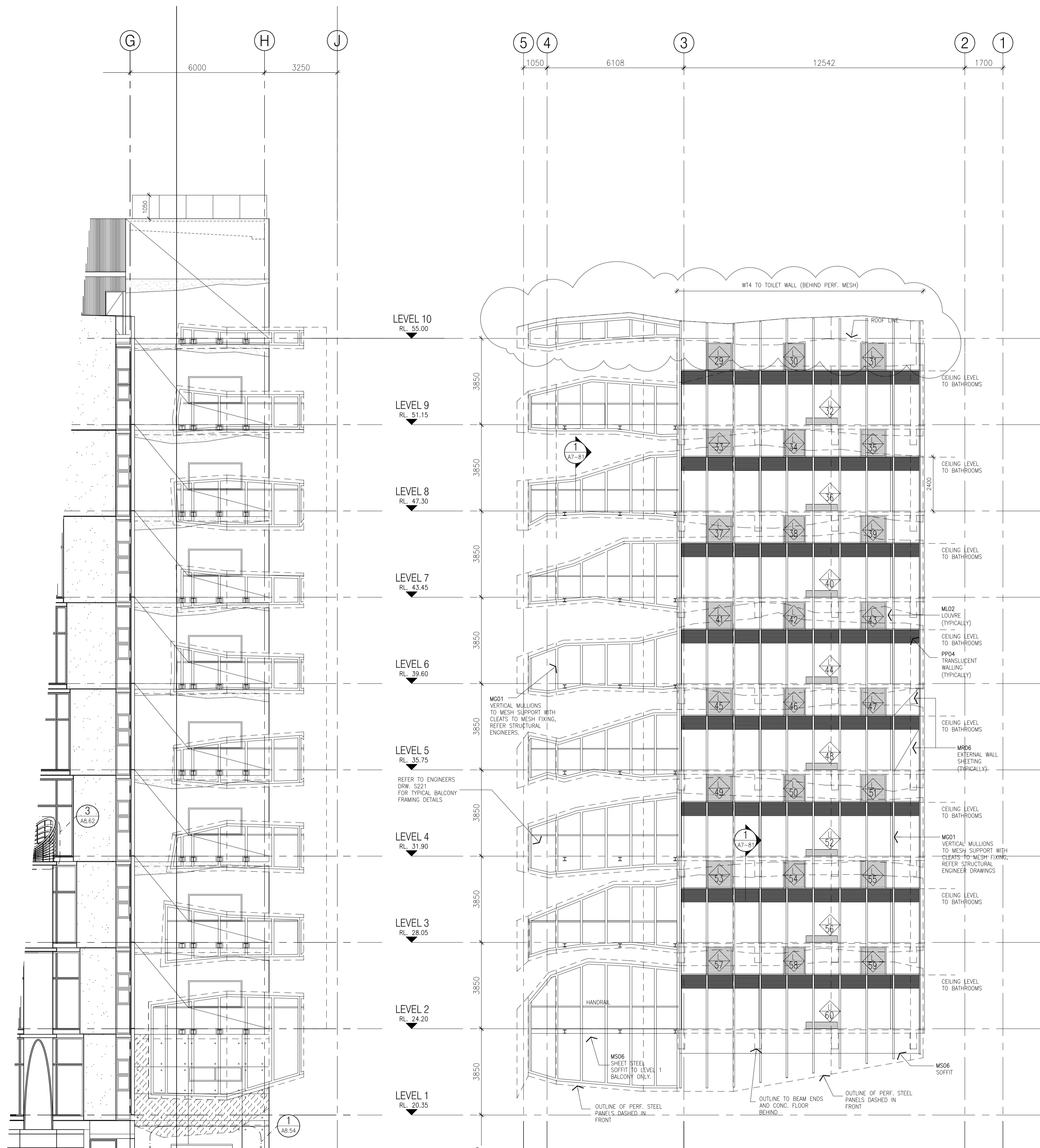
01 SOUTH ELEVATION - EAST BALCONY FRAMING TO PERFORATED MESH SCALE 100
